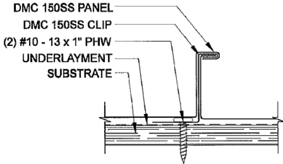
(Field Condition Seam Detail)
